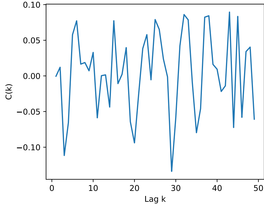
HOMO Autocorrelation
